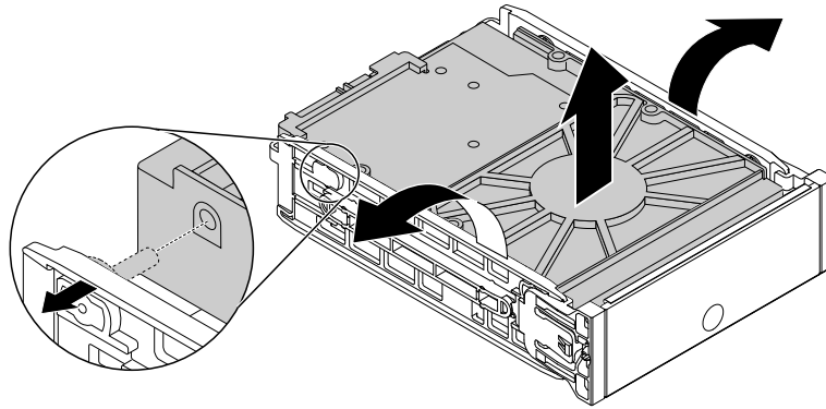
Figure 48. Removing the storage drive from the type 2 bracket
