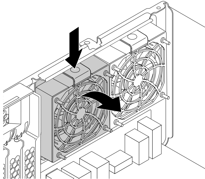
Figure 103. Removing the rear fan assembly
