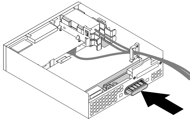
Figure 20. Removing the slim optical drive from the flex module
