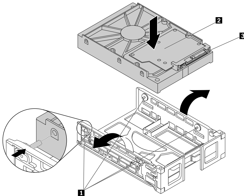
Figure 45. Installing the storage drive into the type 1 bracket
