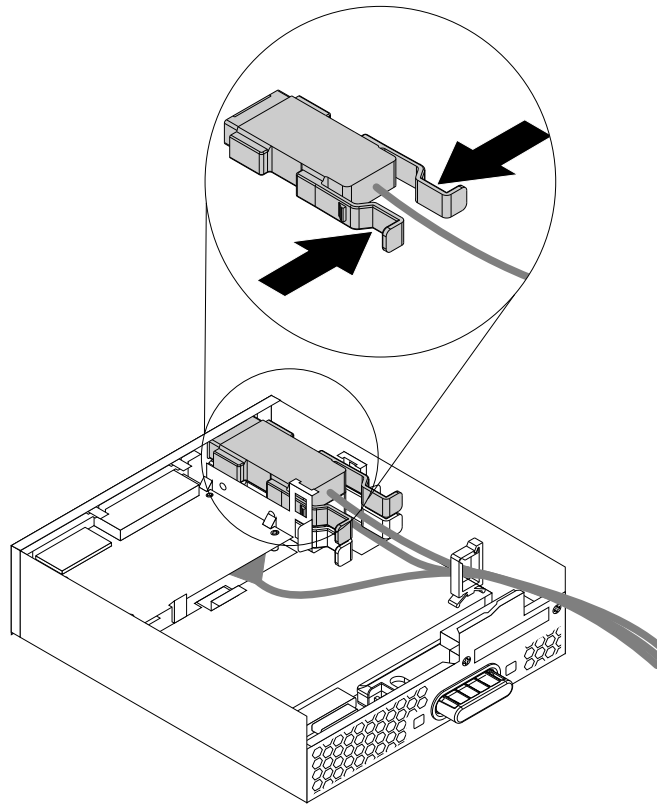
Figure 32. Removing the eSATA connector or IEEE 1394 connector in the flex module
