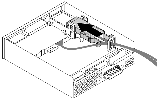
Figure 33. Installing the eSATA connector or IEEE 1394 connector in the flex module
