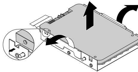
Figure 70. Removing the storage drive from the metal bracket of the converter
