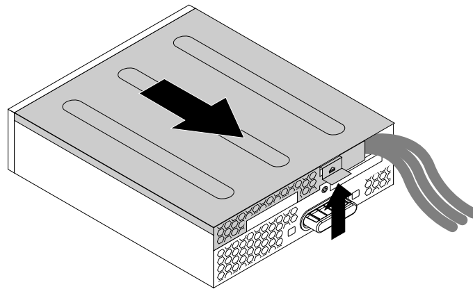
Figure 18. Removing the flex module cover
