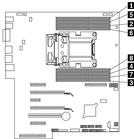
Figure 107. Memory module installation order for ThinkStation P500
