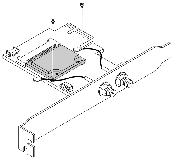
Figure 121. Removing the screws that secure the Wi-Fi card module
