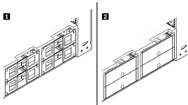
Figure 42. Two types of storage drive bracket
