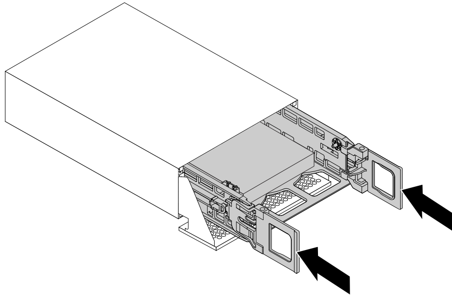
Figure 84. Installing the storage drive bracket
