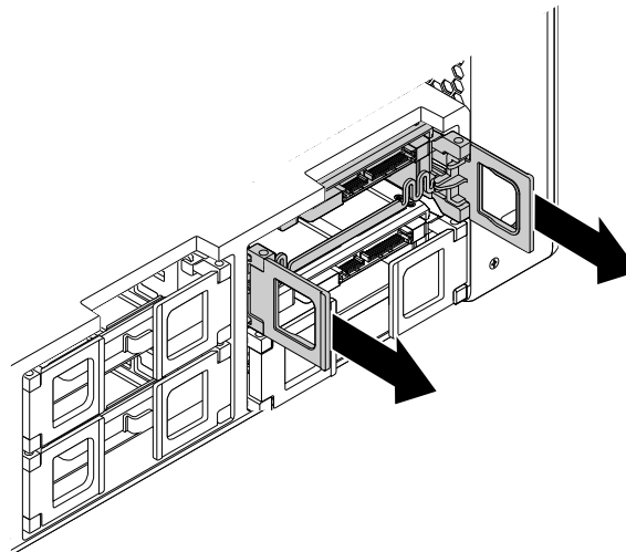
Figure 58. Removing the type 1 storage drive bracket
