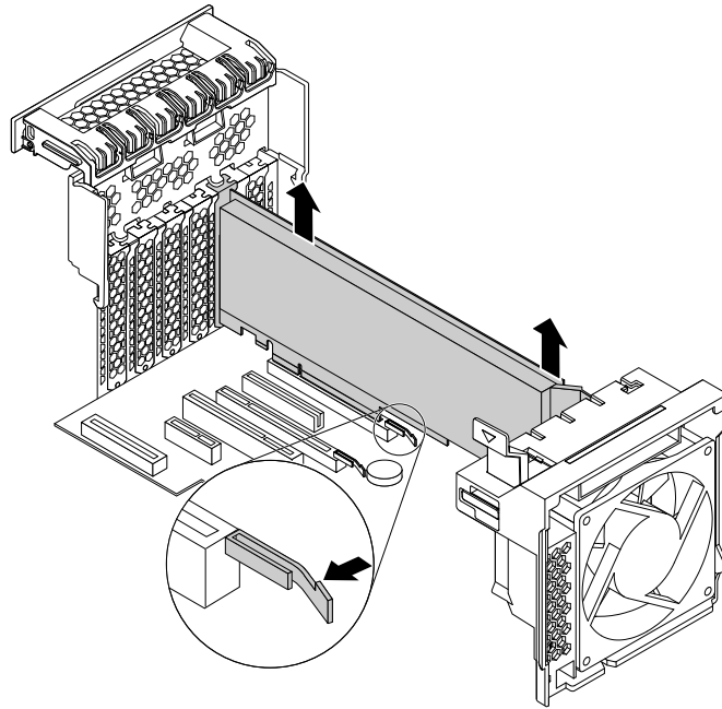
Figure 99. Removing a full-length PCI card
