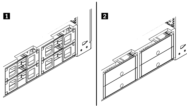
Figure 57. Two types of storage drive bracket
