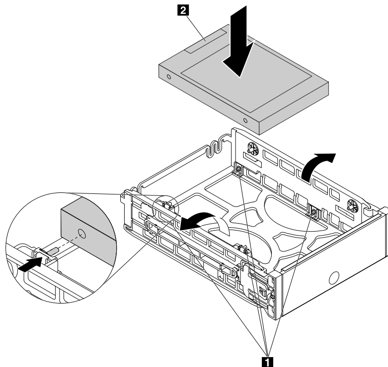
Figure 64. Installing the storage drive into the type 2 bracket
