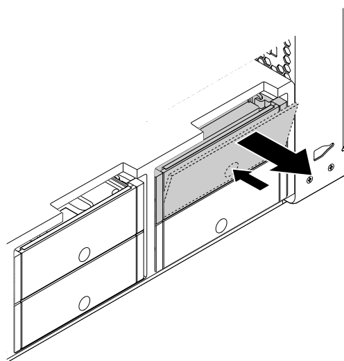
Figure 62. Removing the type 2 storage drive bracket
