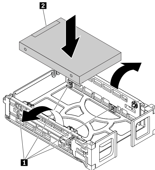
Figure 83. Installing the storage drive into the bracket
