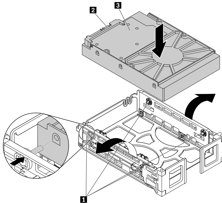
Figure 54. Installing the storage drive into the bracket
