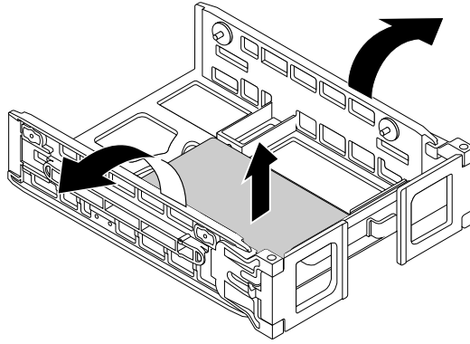
Figure 59. Removing the storage drive from the type 1 bracket
