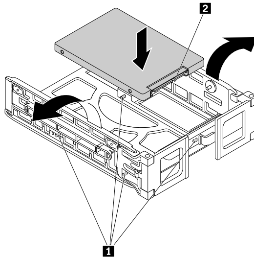
Figure 60. Installing the storage drive into the type 1 bracket
