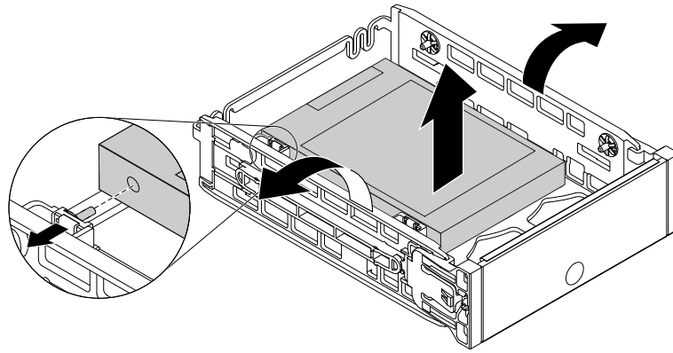
Figure 63. Removing the storage drive from the type 2 bracket
