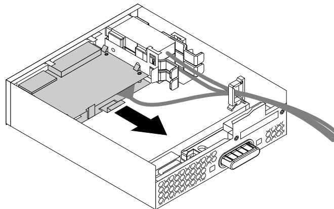
Figure 26. Removing the card reader in the flex module
