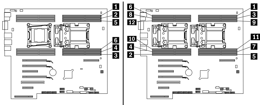
Figure 108. Memory module installation order for ThinkStation P700
