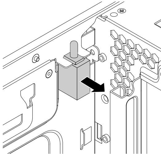
Figure 38. Removing the cover presence switch
