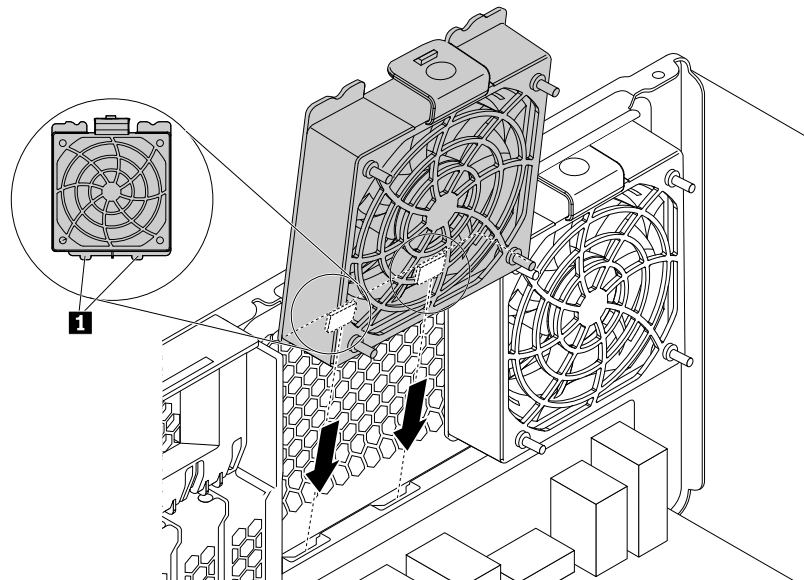
Figure 104. Positioning the rear fan assembly
