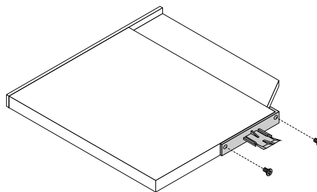
Figure 22. Installing the plastic clip to the slim optical drive
