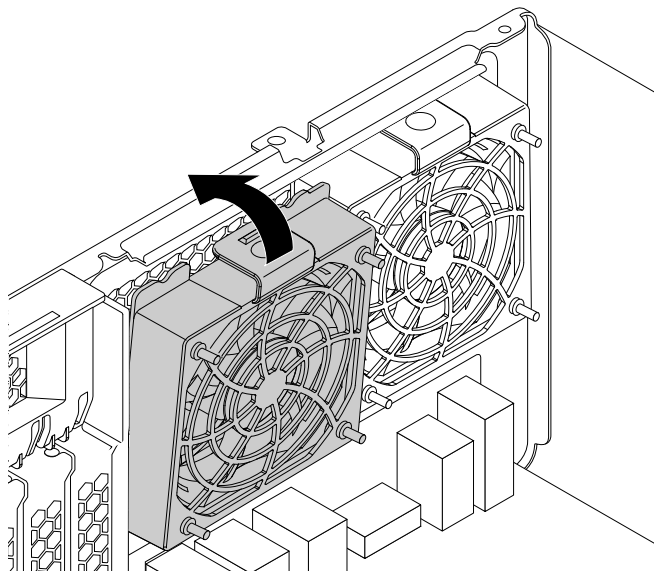
Figure 105. Installing the rear fan assembly
