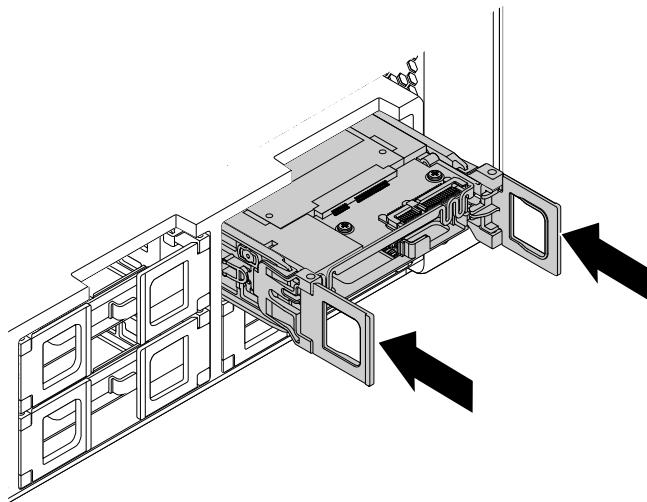
Figure 75. Installing the type 1 storage drive bracket
