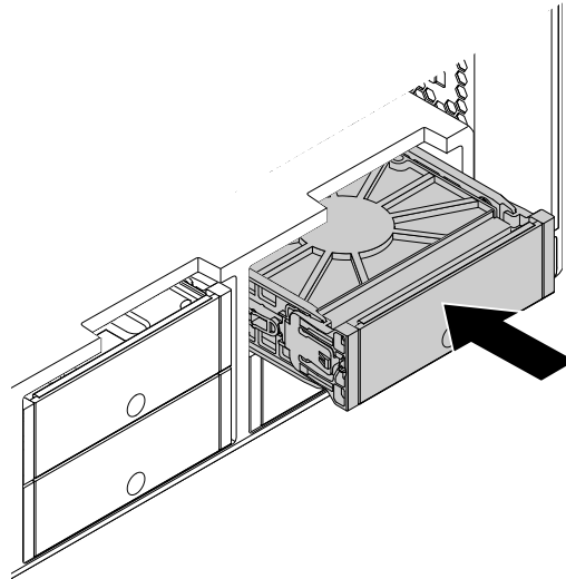
Figure 50. Installing the type 2 storage drive bracket
