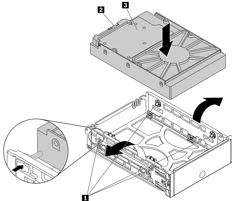
Figure 49. Installing the storage drive into the type 2 bracket
