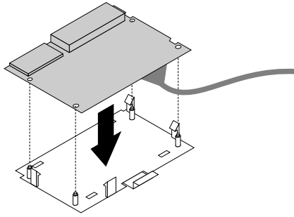
Figure 28. Installing the card reader into the card reader retaining bracket
