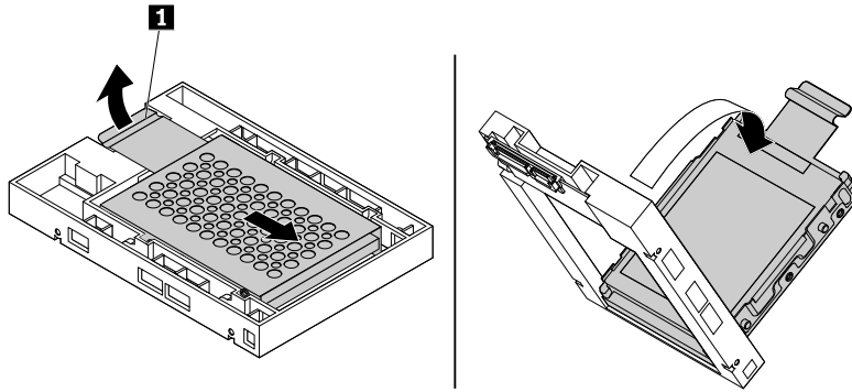
Figure 69. Removing the metal bracket from the plastic frame of the converter
