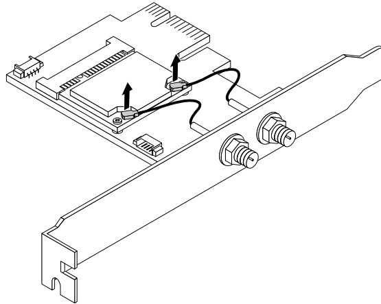
Figure 120. Disconnecting the Wi-Fi antenna cables
