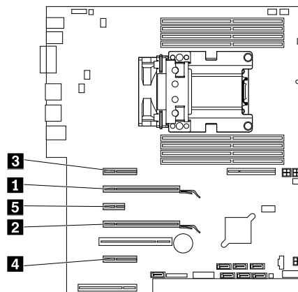
Figure 90. PCI Express card installation order for ThinkStation P500
