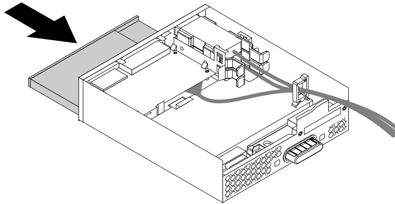
Figure 23. Installing the slim optical drive in the flex module
