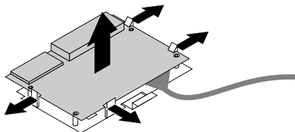
Figure 27. Removing the card reader from the card reader retaining bracket
