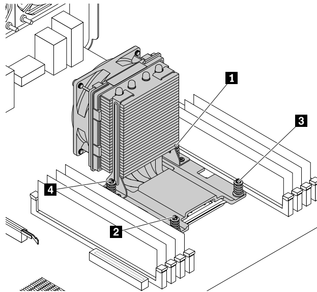
Figure 106. Removing the heat sink and fan assembly
