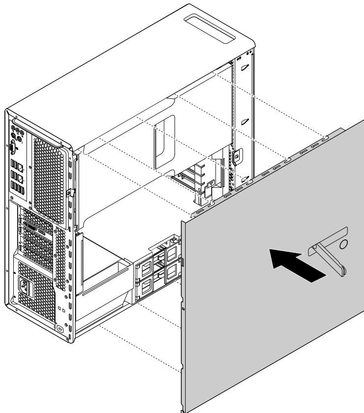
Figure 130. Positioning the computer cover
