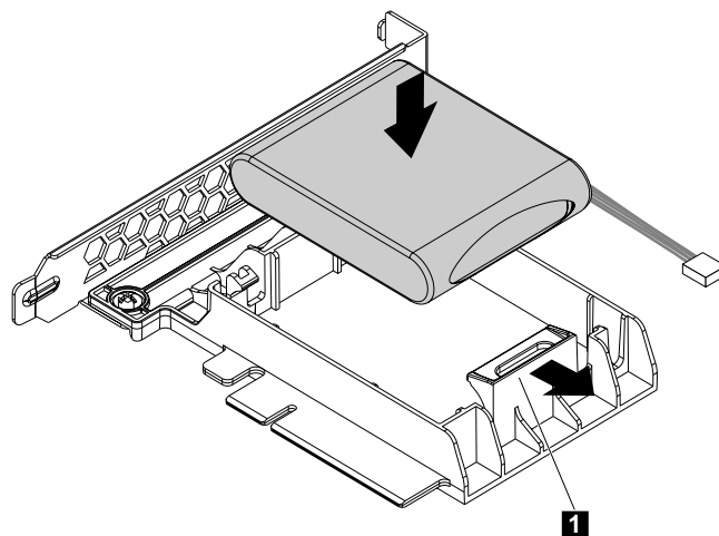
Figure 101. Installing the super capacitor module into the bracket
