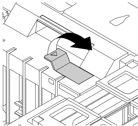
Figure 92. Opening the latch in the front fan assembly
