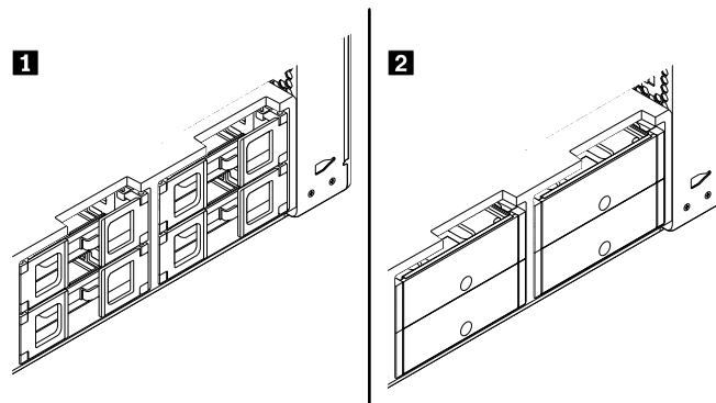
Figure 66. Two types of storage drive bracket
