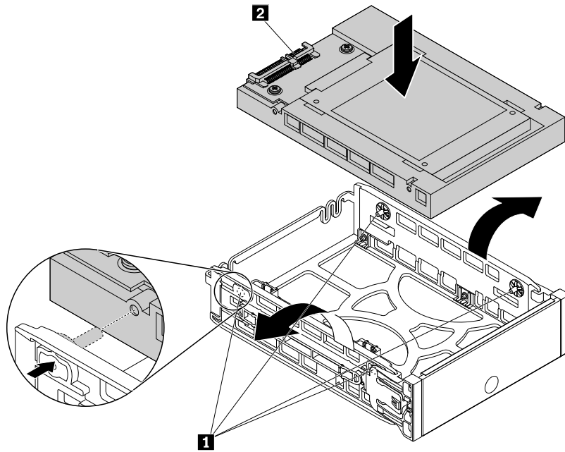
Figure 78. Installing the converter into the type 2 bracket
