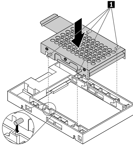
Figure 72. Inserting the metal bracket into the plastic frame of the converter
