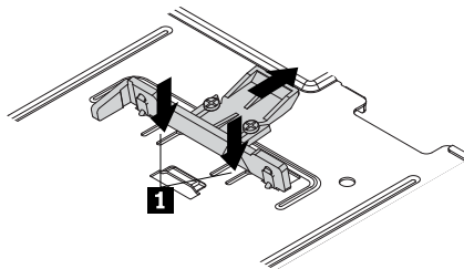
Figure 19. Removing the plastic clip with the two screws
