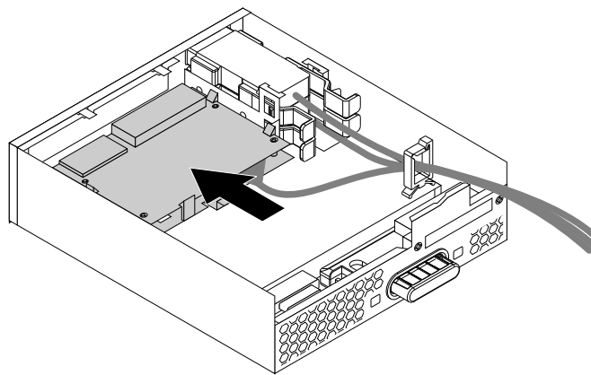
Figure 29. Installing the card reader in the flex module
