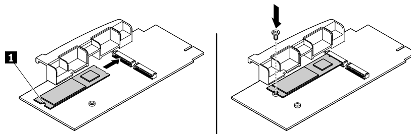
Figure 87. Installing the M.2 solid-state drive
