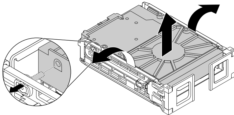
Figure 53. Removing the storage drive from the bracket
