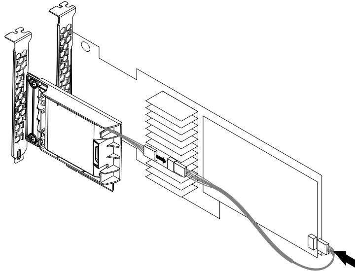
Figure 102. Connecting the super capacitor module cable
