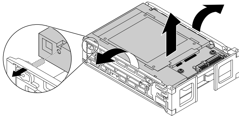
Figure 68. Removing the converter from the type 1 bracket
