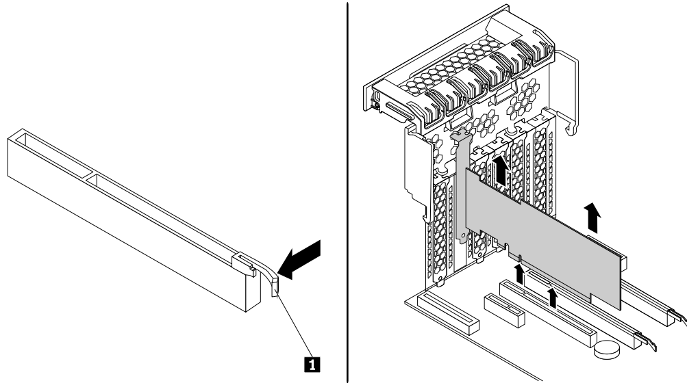
Figure 95. Removing a PCI card
