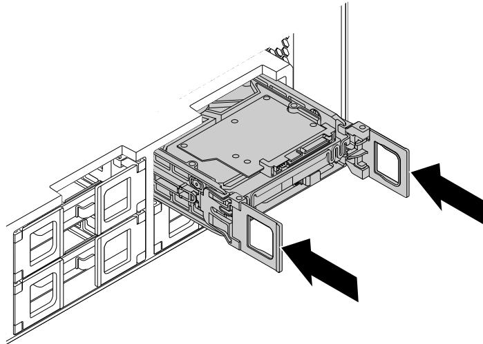
Figure 46. Installing the type 1 storage drive bracket
