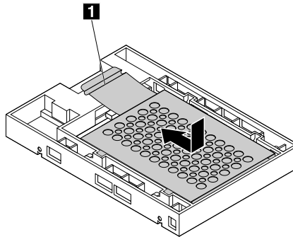
Figure 73. Installing the metal bracket into the plastic frame of the converter
