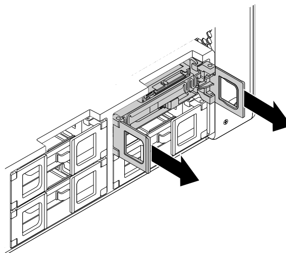
Figure 43. Removing the type 1 storage drive bracket
