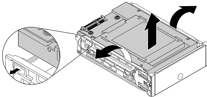
Figure 77. Removing the converter from the type 2 bracket
