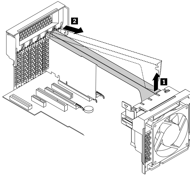
Figure 93. Removing the PCI card retainer
