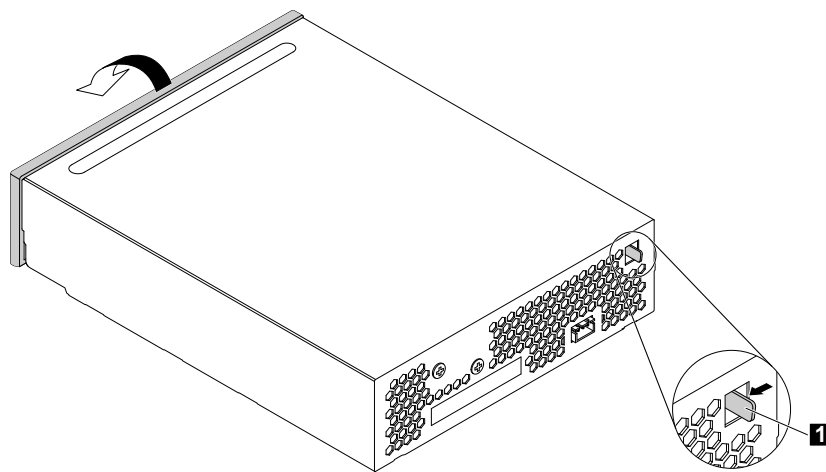
Figure 51. Opening the front cover of the front-access storage enclosure
