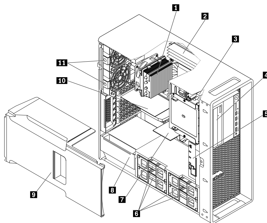
Figure 4. Component locations
