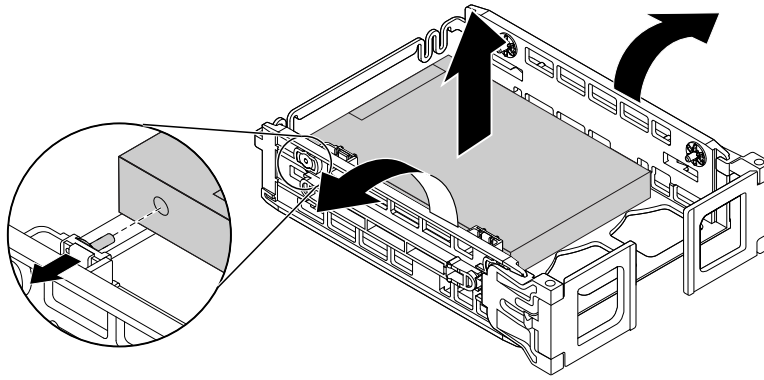
Figure 82. Removing the storage drive from the bracket
