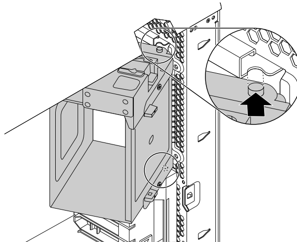
Figure 36. Positioning the optical drive bracket into the chassis
