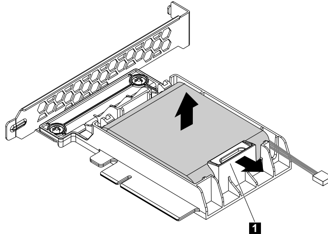
Figure 100. Removing the super capacitor module from the bracket
