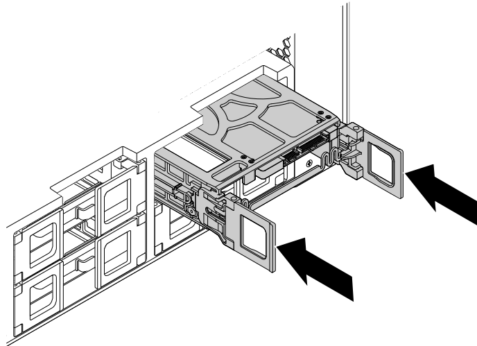
Figure 61. Installing the type 1 storage drive bracket
