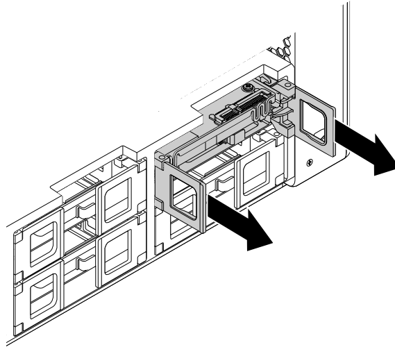
Figure 67. Removing the type 1 storage drive bracket
