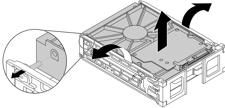
Figure 44. Removing the storage drive from the type 1 bracket
