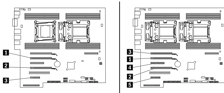
Figure 91. PCI Express card installation order for ThinkStation P700
