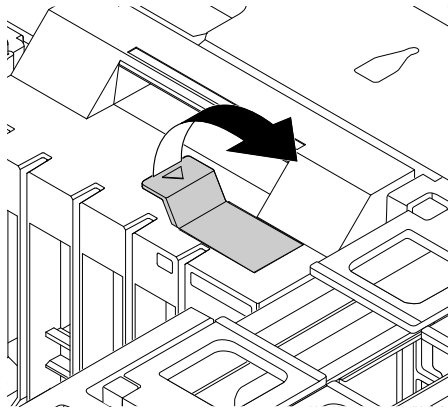
Figure 98. Opening the latch in the front fan assembly
