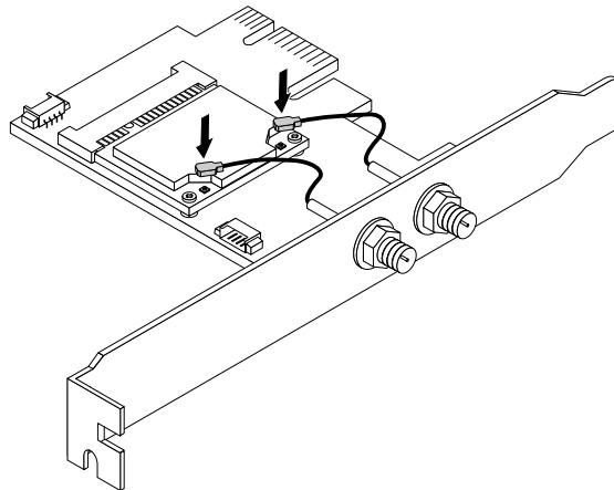
Figure 125. Installing the Wi-Fi antenna cables
