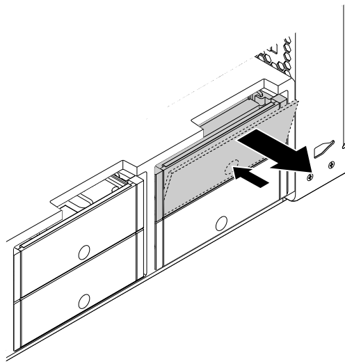
Figure 76. Removing the type 2 storage drive bracket
